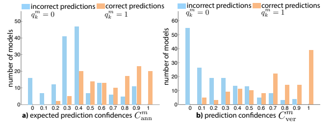
Figure 5: Given a dataset of models with ground-truth human verifications Q^m , we demonstrate the distribution of our prediction confidences, C^m (x-axis) (blue bars for incorrectly propagated predictions and brown for correct). A good confidence predictor is expected to place higher blue bars closer to 0 on the x-axis, correctly identifying the bad predictions, and higher yellow bars closer to 1 on the x-axis, correctly identifying the good predictions. (a) While the estimates used to select the annotation set in the beginning, i.e. with no human input yet, are less accurate, they are sufficient to bootstrap our algorithm. (b) These estimates significantly improve after a single iteration of annotation propagation enabling to optimize for a more reliable verification set.
