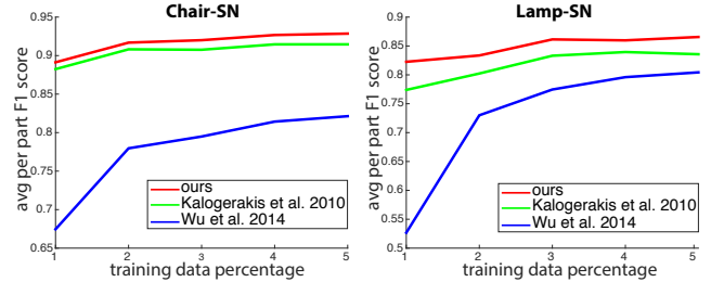
Figure 12: Our automatic label propagation tool demonstrates a superior performance in comparison to previous techniques (adapted to handle ShapeNetCore data).
