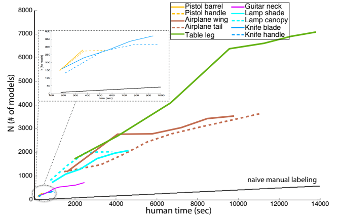
Figure 10: Number of positively-verified labeled shapes ( y -axis) as a function of human input time ( x -axis) for representative labels in our data. As expected the graph is monotonically increasing, and flattens out as time progresses and the algorithm encounters more diverse models. Note the relative inefficiency of manual labeling.
