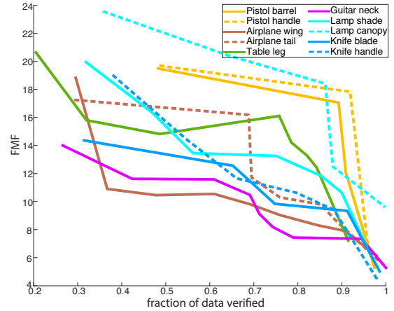
Figure 11: Force-multiplication factor (FMF, y -axis) over time. Predictably FMF drops as the system annotates a higher fraction of the model collection ( x -axis).
