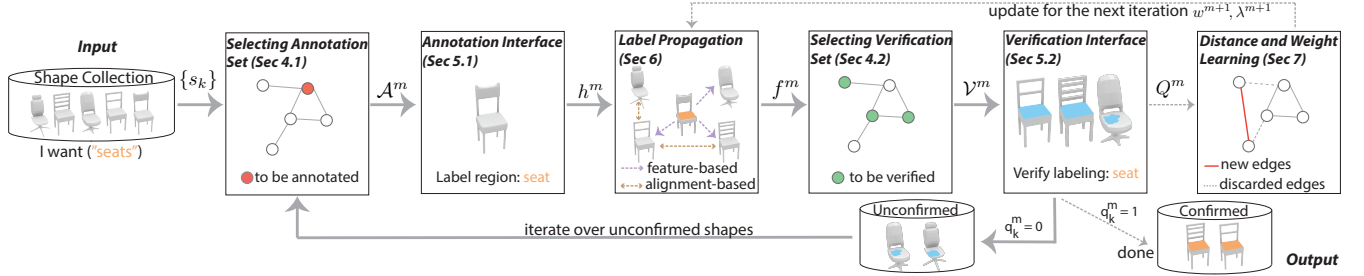
Figure 3: This figure summarizes our pipeline. Given the input dataset we select annotation set and use our UI to obtain human labels. We automatically propagate these labels to the rest of the shapes and then query the users to verify most confident propagations. We then use these verifications to improve our propagation technique.
