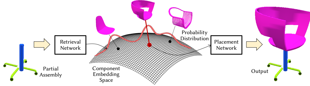
Fig. 2. Overview of the retrieval process at test time. From the given partial assembly, the retrieval network predicts a probability distribution (modeled as a mixture of Gaussians) over the component embedding space. Suggested complementary components are sampled from the predicted distribution, and then the placement network predicts their positions with respect to the query assembly.
