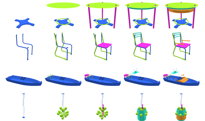
Fig. 12. Failure examples. 1st row: the bottom components match a single leg, but triple legs are retrieved. 2nd row: Green and blue components partially overlap. 3rd row: A sky-blue component is floating. 4th row: Components overlap.
