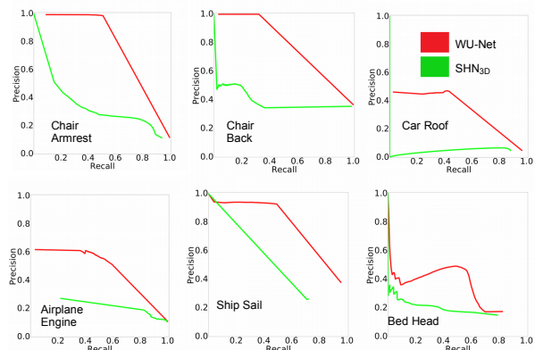
Figure 1: WU-Net (red) consistently outperforms a Stacked Hourglass Network SHN 3D (3 deep U's without low resolution skip connections between different U's, green) on all categories (on training shapes, outputs symmetrized).
