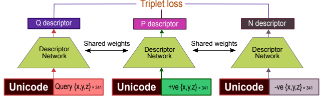
Figure 6: Shape correspondence training setup. Two corresponding points and one mismatched point, whose coordinates are concatenated with the unicodes of their parent shapes, are independently mapped to descriptors by a network, followed by a triplet loss.
