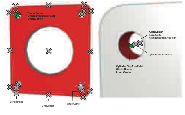
Fig. 10. MCF data augmentation. The red face is the selected orientation topology. Green Xs are MCFs equivalent to the ground truth, and grey Xs are other MCFs that can be constructed from those selections, which are used to construct negative location examples. Selected MCFs have been annotated with their location topology and origin types. Note that there are multiple locations aliasing the ground truth MCFs for both selections.
